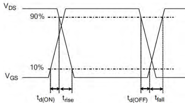
Resistive Switching Waveforms
