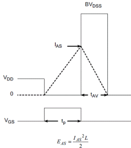
Unclamped Inductive Switching Waveform
