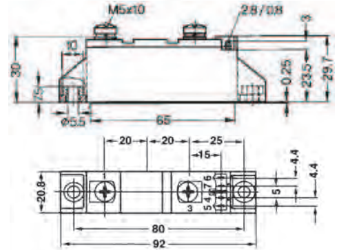
Dimensions in mm (1mm=0.0394")
